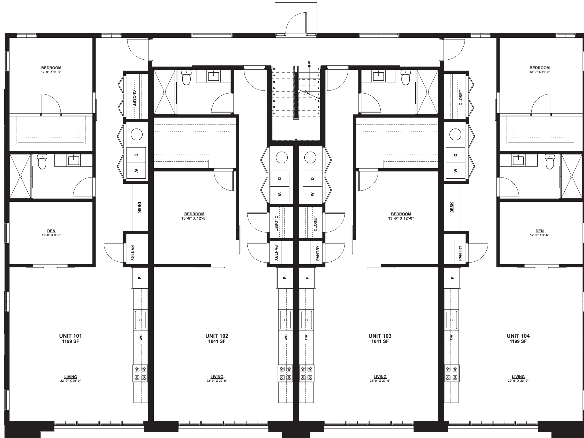
SECOND FLOOR RESIDENCE FLOOR PLAN / 4 UNITS - NTS
