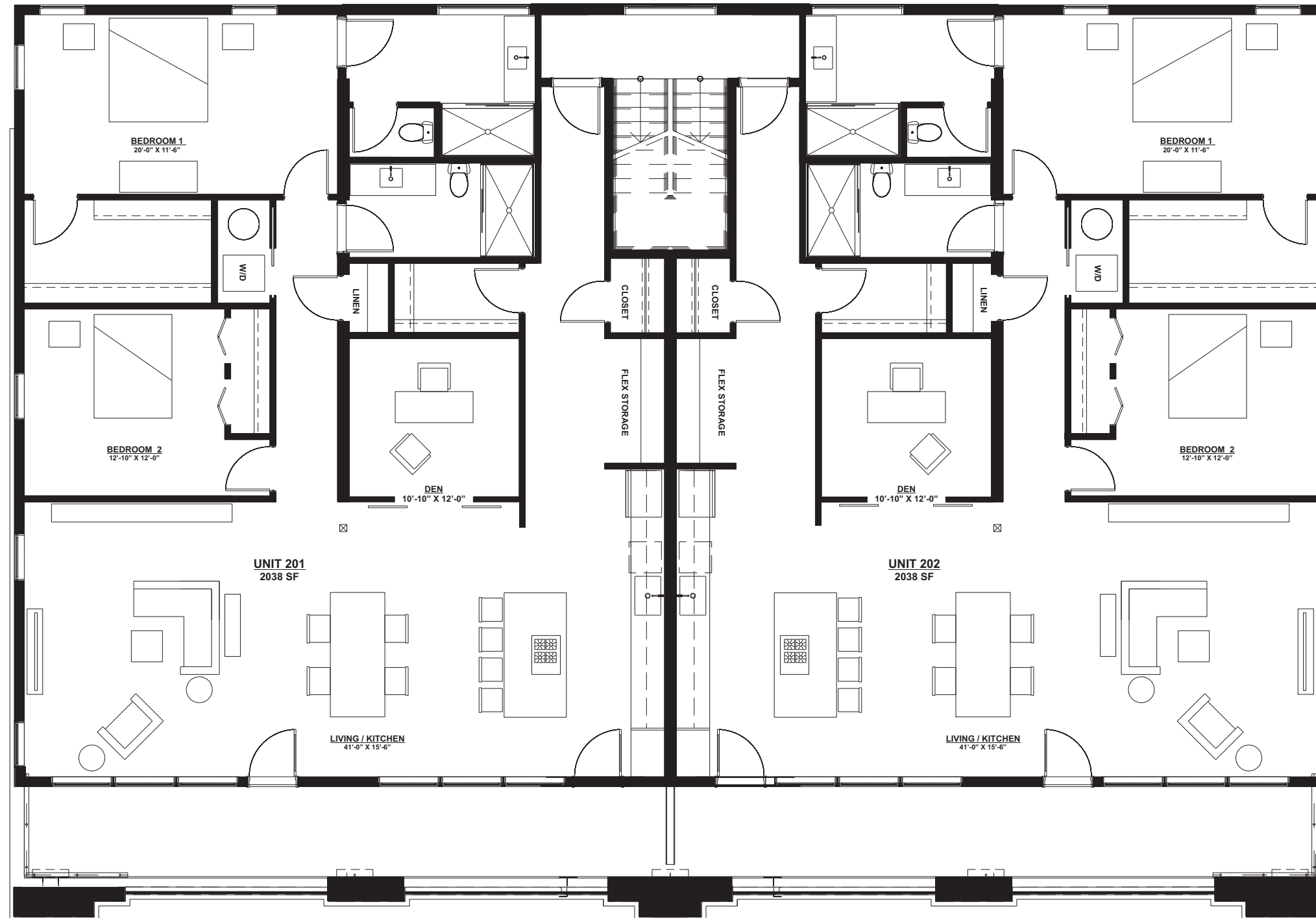
THIRD FLOOR RESIDENCE FLOOR PLAN / OPTIONAL 2 UNITS - NTS
