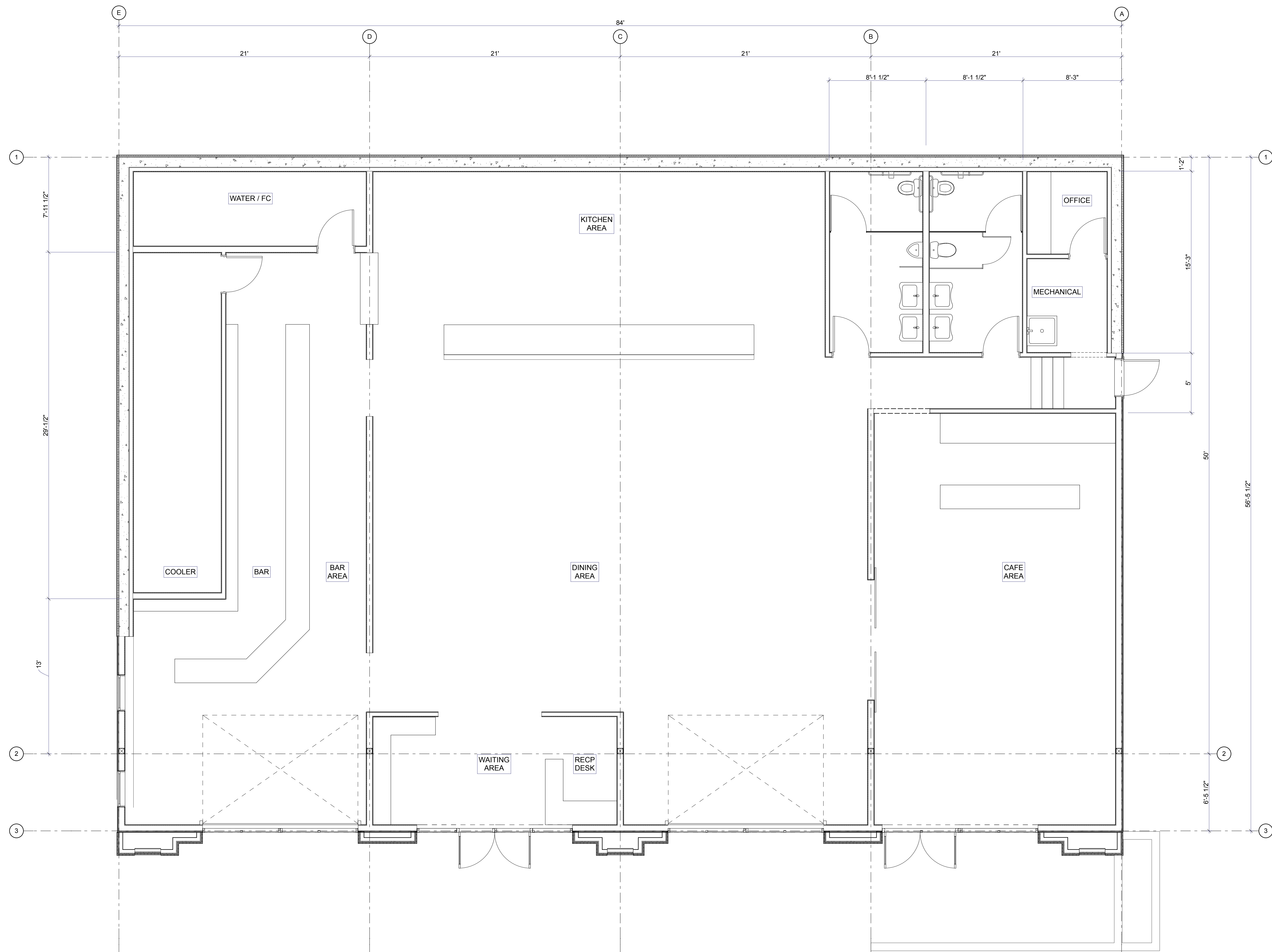
1 Restaurant Level SCALE: 1/4" = 1'-0"
