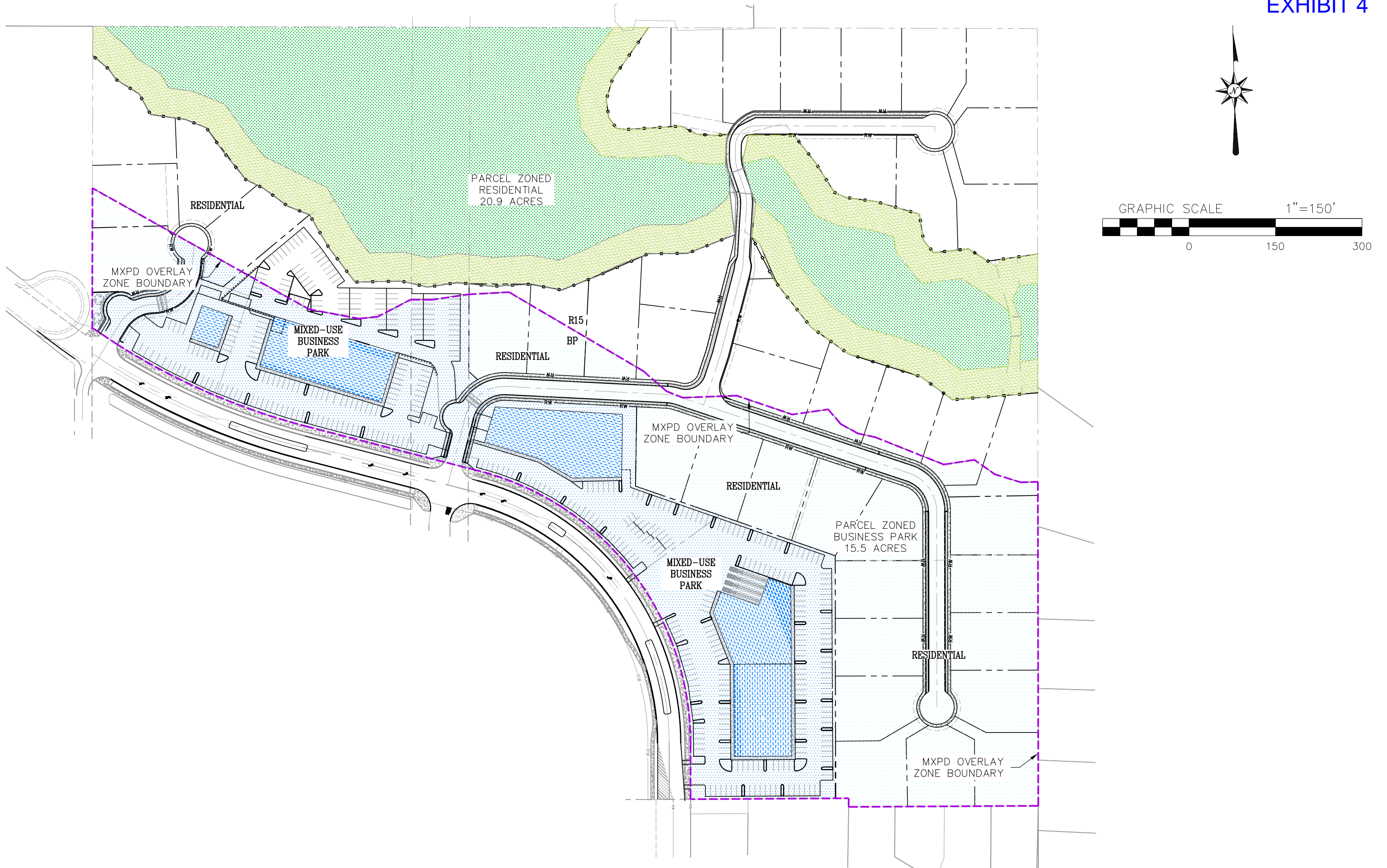
PROPOSED MXPd OVERLAY MAP
