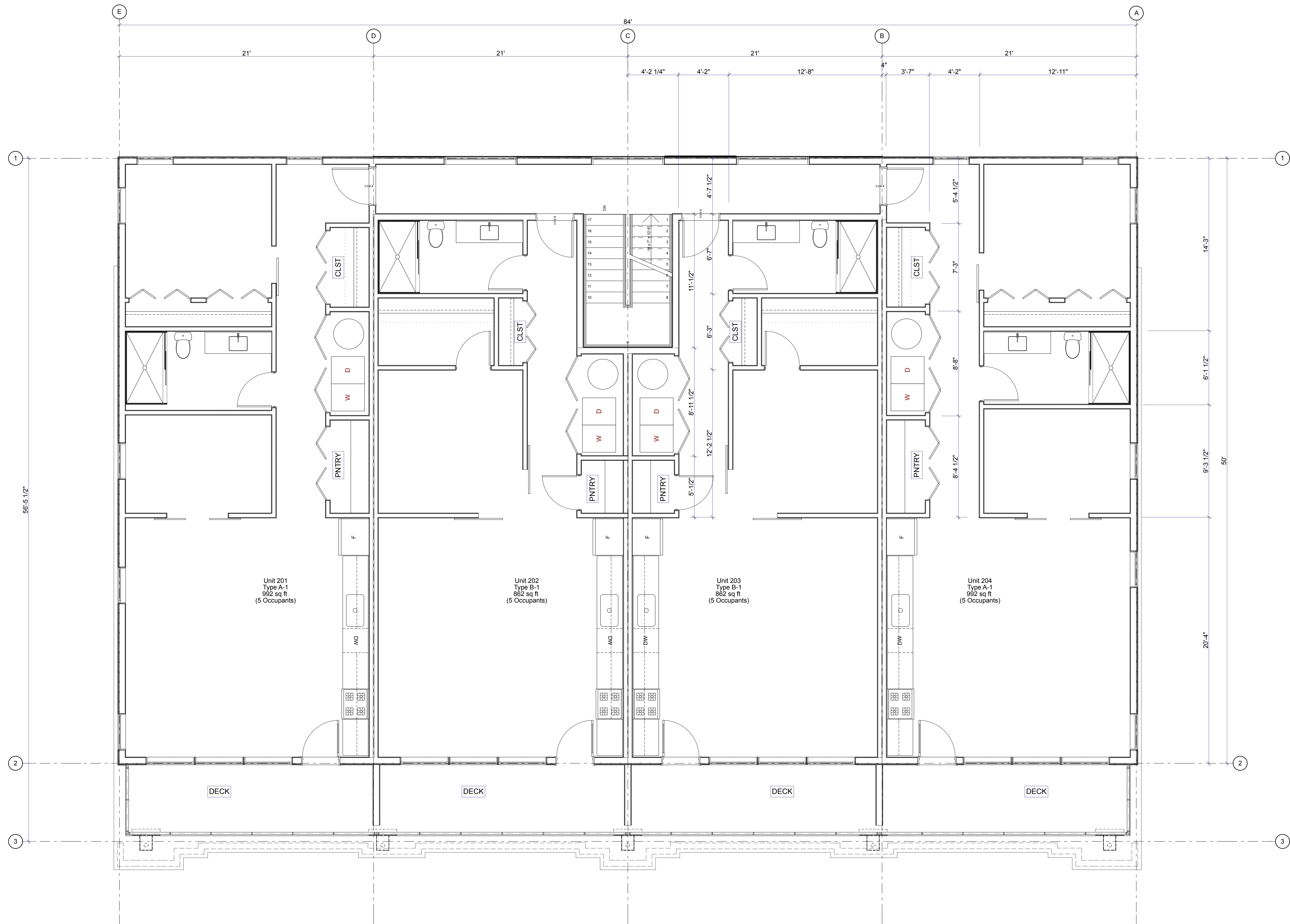
1 Residential Level 2 SCALE: 1/4" = 1'-0"
